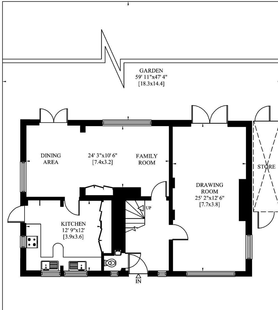
GROUND FLOOR
