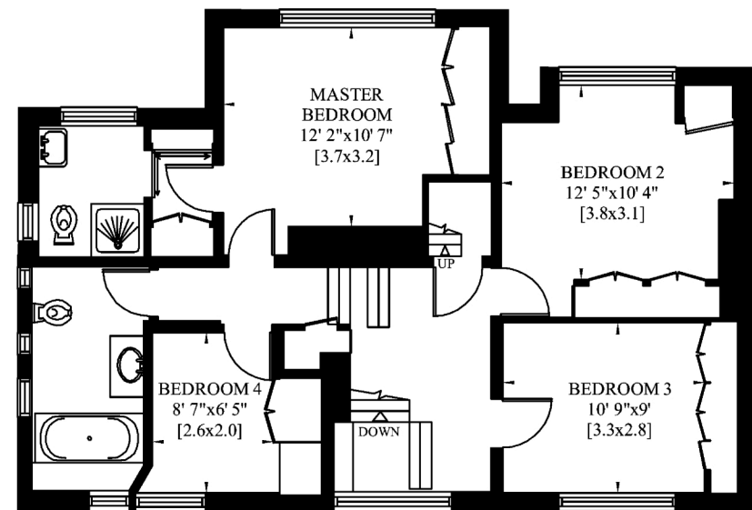
SECOND FLOOR
