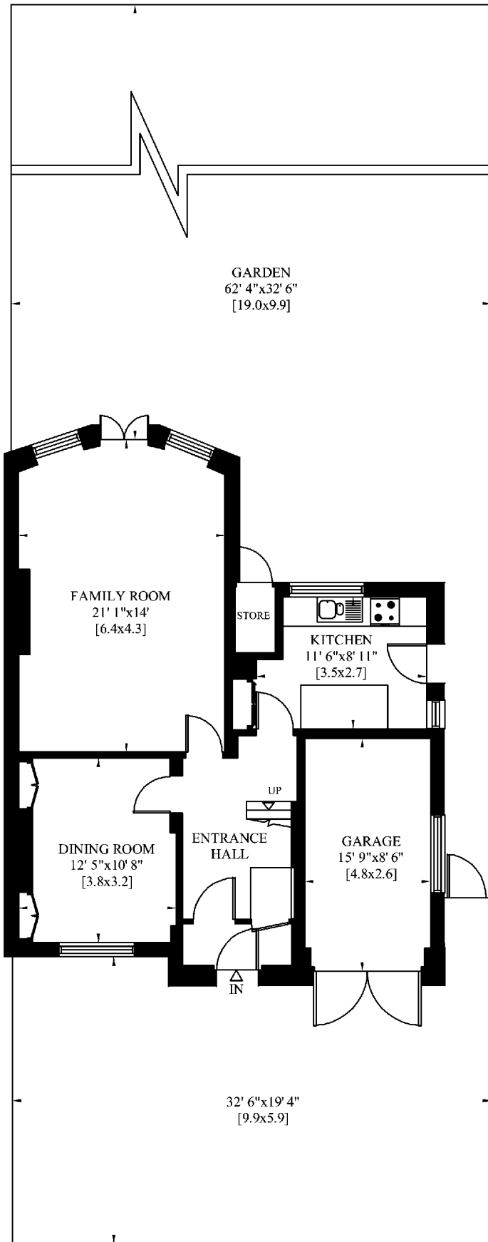
GROUND FLOOR
