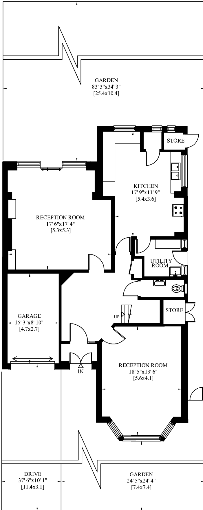
GROUND FLOOR
