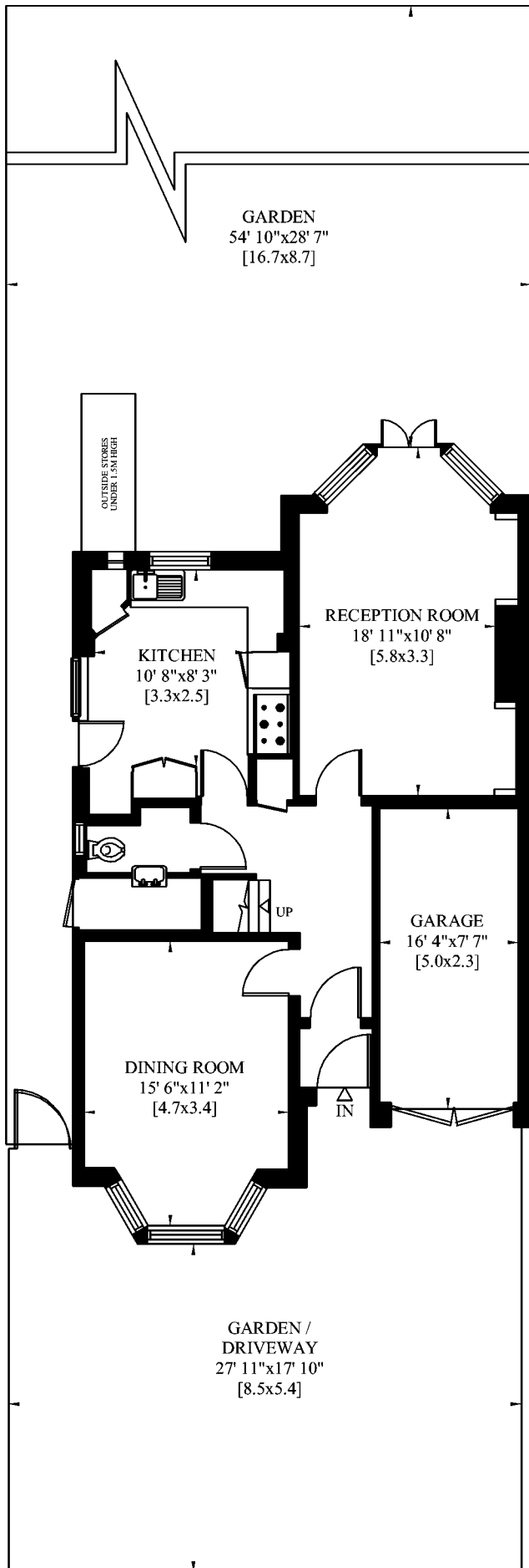
GROUND FLOOR
