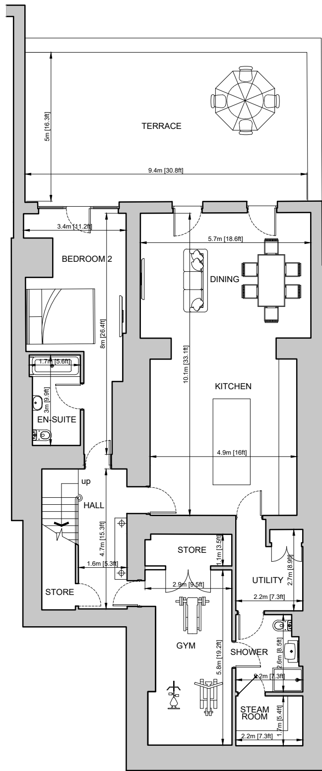
LOWER GROUND FLOOR PLAN
